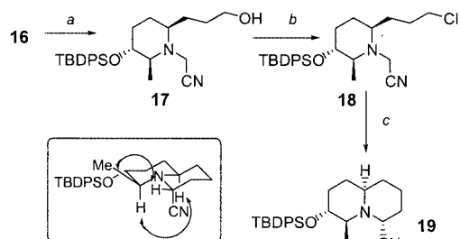
Scheme 2. Reagents and conditions: (a) \text{BrCH}_2\text{CN} , \text{K}_2\text{CO}_3 , \text{CH}_3\text{CN} , reflux, 93%. (b) \text{SOCl}_2 , DCM, reflux. (c) \text{LiHMDS} , THF, -78^\circ\text{C} , 89% overall
