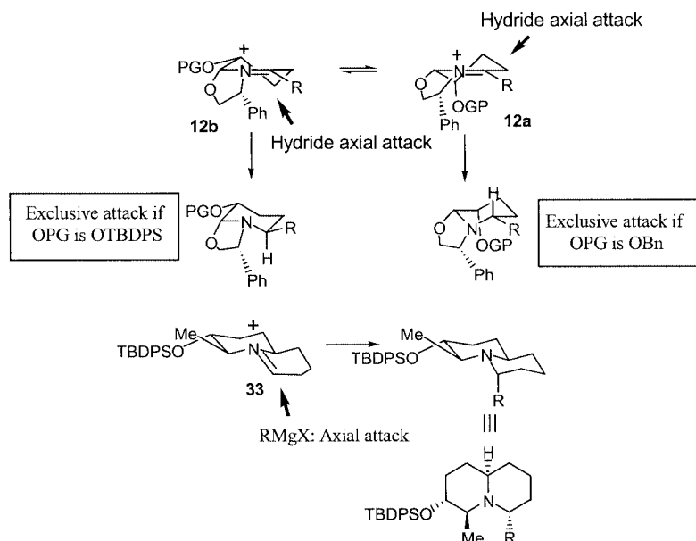
Figure 5. The stereoselectivity of the reduction of amino nitrile 13 and of the alkylation of amino nitrile 19 can be explained by stereoelectronic effects that govern the attack of intermediate iminium ions
