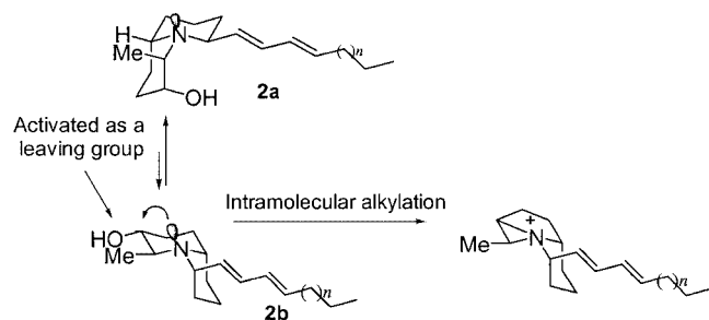
Figure 2. A putative mechanism involving generation of electrophilic aziridinium ions from clavepictines
