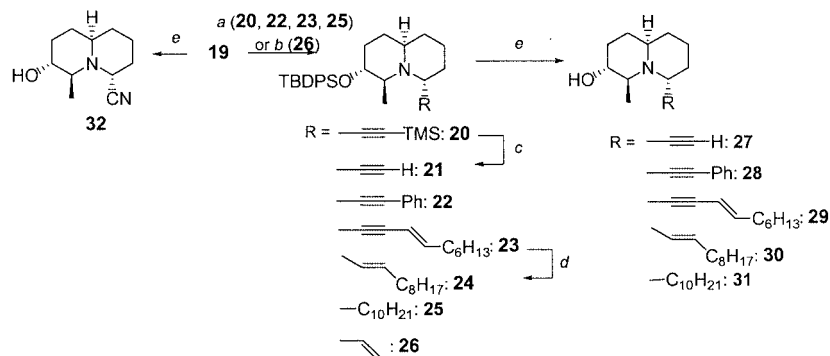
Scheme 3. Reagents and conditions: (a) \text{RMgBr} , THF, room temperature, quant. ( 20 ), 89% ( 22 ), 84% ( 23 ), 93% ( 25 ). (b) \text{AgBF}_4 , THF, room temperature, then vinylmagnesium bromide, -78 to 0^\circ\text{C} , 80%. (c) \text{K}_2\text{CO}_3 , MeOH, quant. (d) \text{Na} , liq. \text{NH}_3 , THF, -78^\circ\text{C} , 51%. (e) TBAF, THF, 50^\circ\text{C} , 68% ( 27 ), 68%, ( 28 ), 77% ( 29 ), 65% ( 30 ), 76% ( 31 ), 84% ( 32 )
