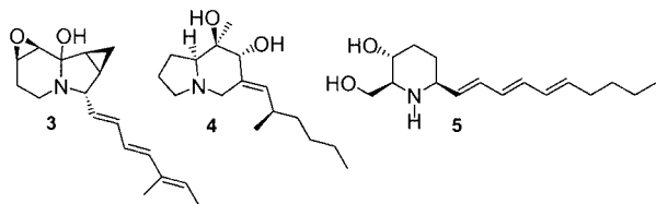
Figure 3. Some alkaloids showing the substructure necessary to generate aziridinium ions
