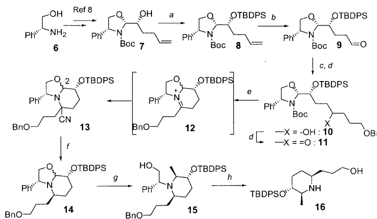
Scheme 1. Reagents and conditions: (a) NaH, THF, then TBDPSCl, 55–60 °C, 92%. (b) OsO 4 (cat.), NaIO 4 , THF/H 2 O, room temperature, 91%. (c) BnO(CH 2 ) 3 MgBr, Et 2 O, room temperature, 98%. (d) (COCl) 2 , DMSO, Et 3 N, DCM, –50 °C, 94%. (e) TFA, DCE, room temperature then KCN/H 2 O, 89%. (f) AgBF 4 , THF, room temperature, then Zn(BH 4 ) 2 , –78 °C, 85%. (g) MeMgBr, THF, room temperature, 89%. (h) H 2 , Pd(OH) 2 , EtOH, quant.
