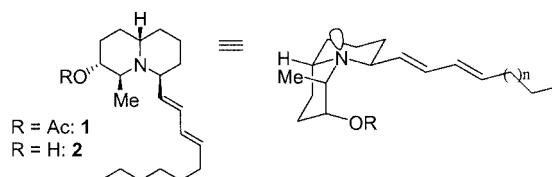
Figure 1. Natural clavepictines isolated from Clavelina picta
